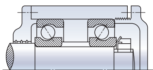
Fig. 10 Preload application by screw
