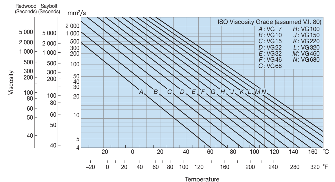
Fig. 22 Temperature-Viscosity chart
