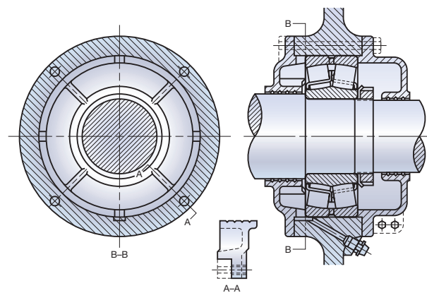
Fig. 25 Grease sectors
