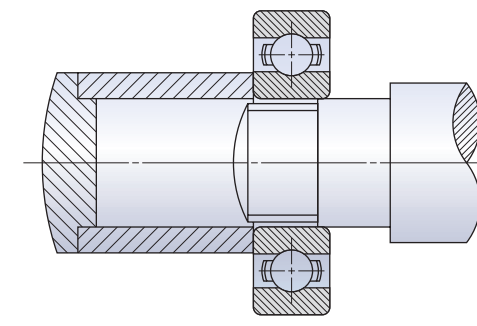
Fig. 3 Mounting of Bearing
