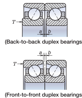
Fig. 15 Amount of preload
