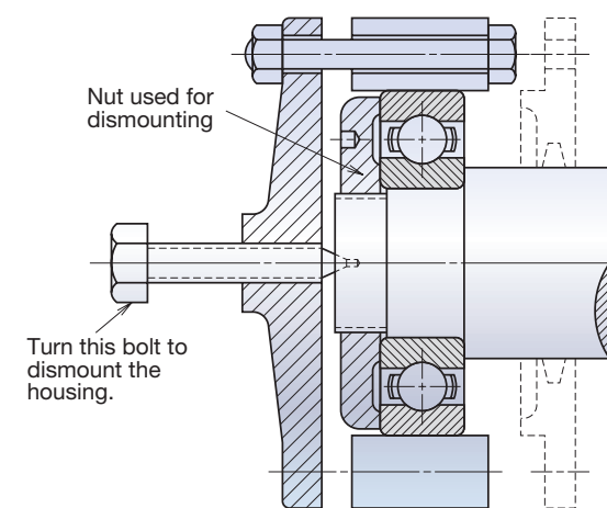
Fig. 42 Dismounting the Outer Ring
