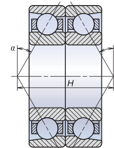
Fig. 14 Back-to-back duplex bearings
