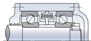
Fig. 11 Preload application by spring
