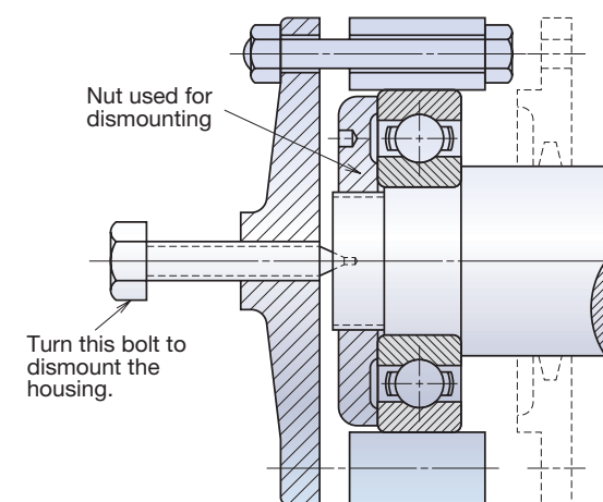
Fig. 42 Dismounting the Outer Ring
