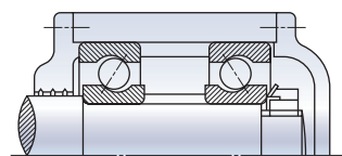
Fig. 12 Preload application by spacer (on free-end)
