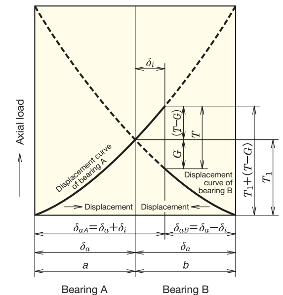
Fig. 16 Axial displacement with preload
