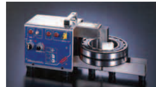
Fig. 5 Heating by bearing heater
