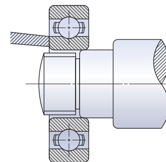
Fig. 2 Mounting of Bearing
