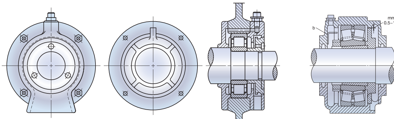
Fig. 26 Grease valve
